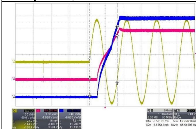
Fig. 5-7, Start-up time is 15.3ms @full load, 230V/50Hz
