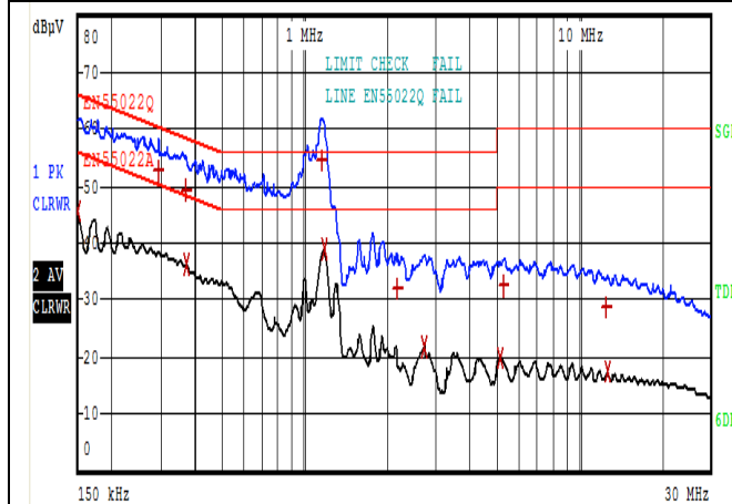
Fig. 5-35, N line conduction waveform@110V, full load.
