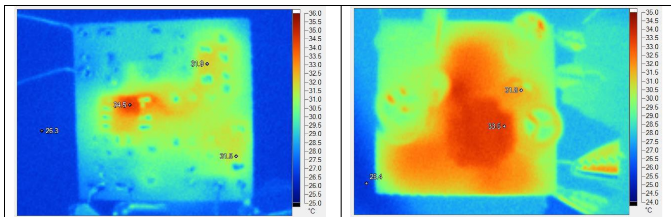
Fig. 5-27, IC 34.5°C, 12V flyback diode 31.5°C, RCD diode 31.9°C@full load, 265V/50Hz, ambient temperature 26.3°C.
