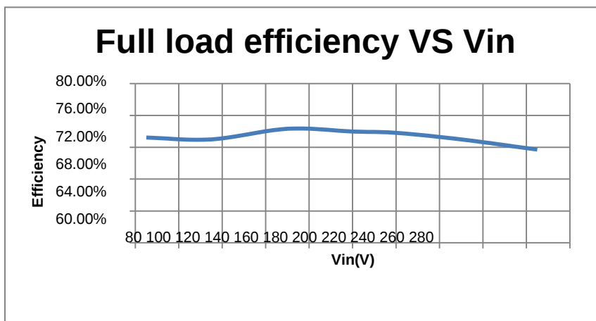
Fig. 5-2, Full load efficiency VS Vin
