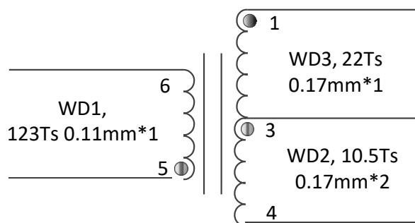
Fig. 3-2, Transformer Electrical Diagram
