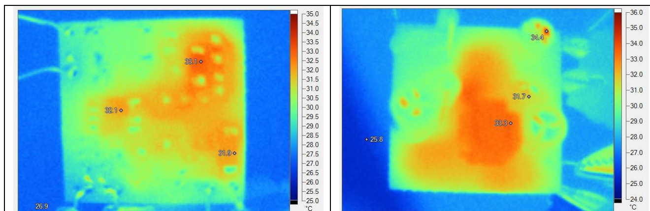
Fig. 5-25, IC 32.1°C, 12V flyback diode 31.9°C, RCD diode 33.1°C@full load, 85V/60Hz, ambient temperature 26.9°C.
